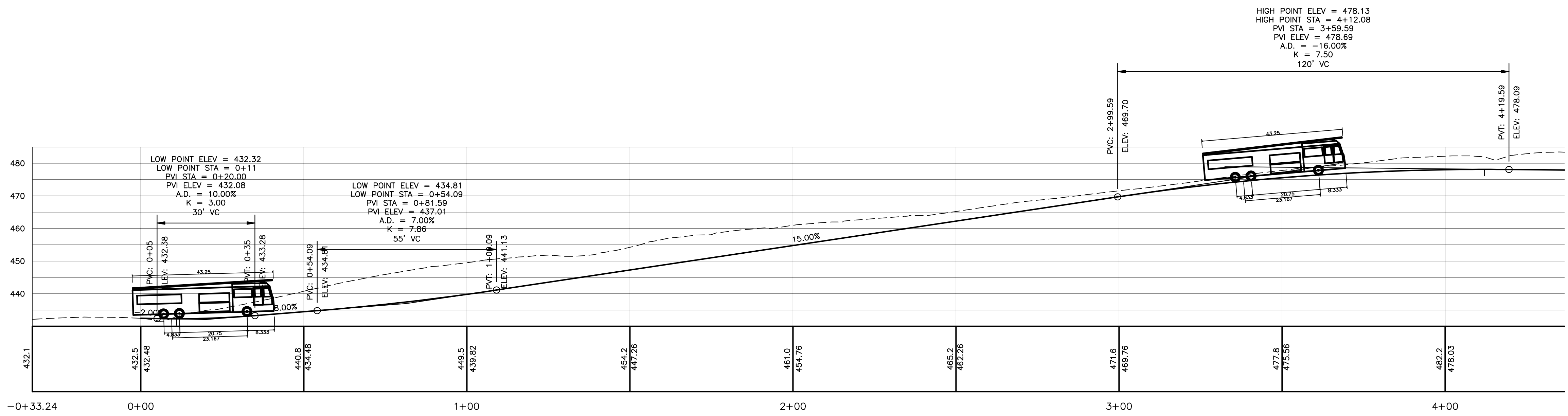
DRIVEWAY PROFILE SCALE: 1" = 20'(HORIZ.) 1" = 10'(VERT.)
